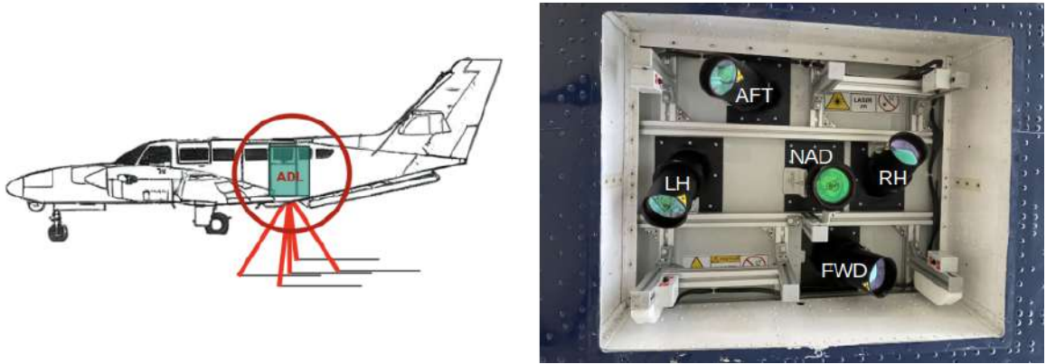
Figure 3.6.: Left: Sketch of the Cessna 406 research aircraft of the Technische Universität Braunschweig with the airborne Doppler lidar (ADL) system AIRflows on board. Right: Photo of the five Doppler lidars of the AIRflows system pointing in fixed directions, photographed from below the aircraft. Courtesy of Dr. Philipp Gasch, combined by the author.
