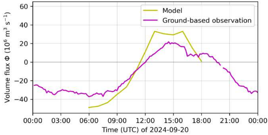
Figure 7.4.: As in Figure 7.3 for 20 September 2024.
