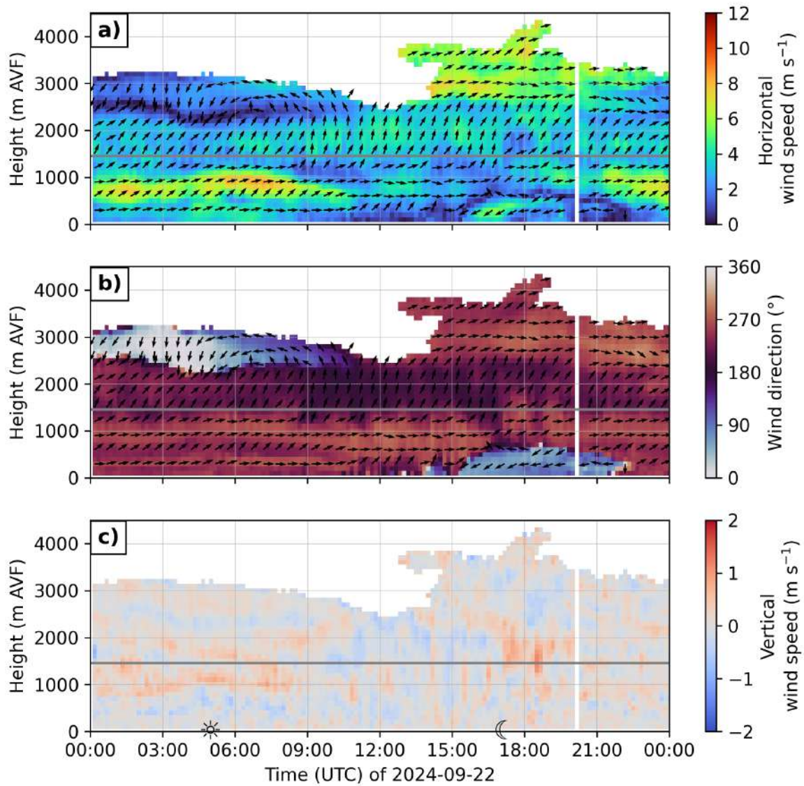
Figure 6.8.: As in Figure 6.2, but for 22 September 2024.
