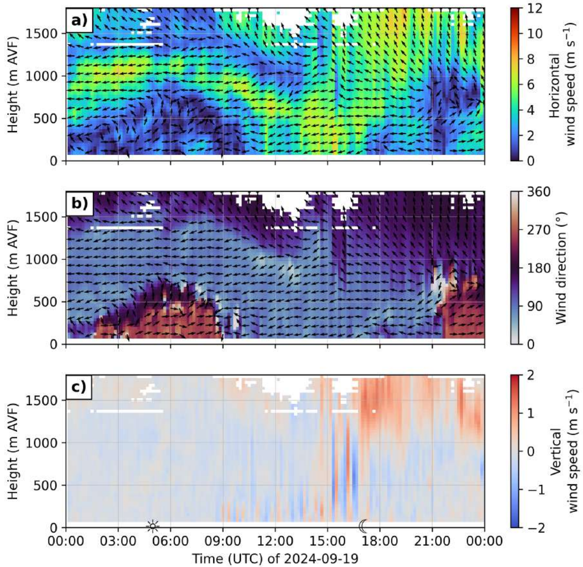
Figure B.1.: Time height plot of Doppler wind lidar observations from Innsbruck for 19 September 2024 showing a) Horizontal wind speed. b) Wind direction. c) Vertical wind speed. Arrows show the wind direction. The sun and moon symbols indicate the sunrise and sunset times. Note the different y-axis range compared to the profiles from Kolsass. Profiles are 10-min averages based on plane position indicator (PPI) scans at 70^{\circ} elevation. The data were kindly provided by the University of Innsbruck, which operates the Doppler lidar.
