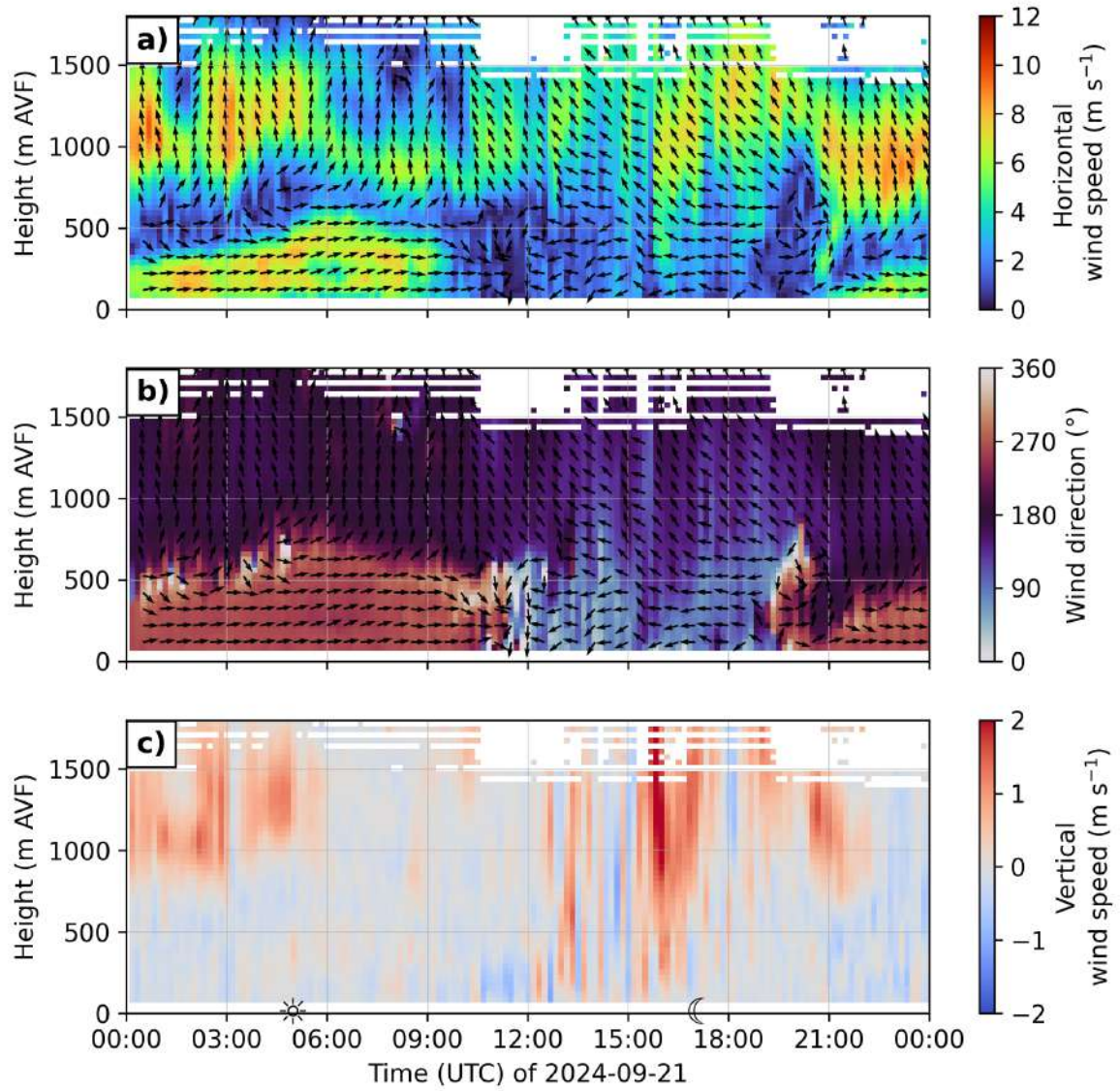
Figure B.3.: As in Figure B.1 but for 21 September 2024.
