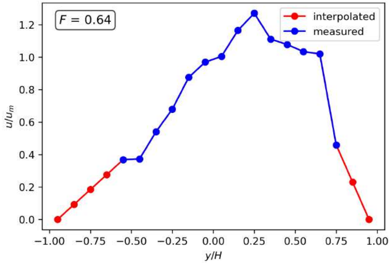
Figure 4.14.: Example weighting factor calculation for three 8° plane position indicator (PPI) scans in down-valley direction on 19 September 2024 at 1001–1041 UTC. Medians of the binned along-valley wind ( u_{\text{along}} ) normalized by the wind speed at the center ( u_m ) as a function of the normalized distance from the valley center ( y/H ). The wind is interpolated towards the side walls with the assumption of zero wind speed at the wall. The resulting weighting factor F is the ratio between the average over the cross-section and the wind speed at the center (average of two central bins).
