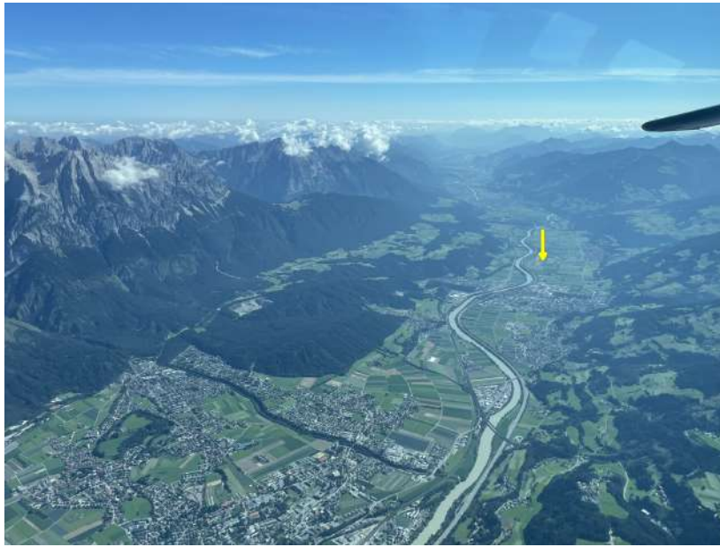
Figure 1.1.: View of the Inn Valley looking northeastward during a measurement flight. The yellow arrow indicates the location of the ground-based Doppler wind lidar in Kolsass. Photo by Philipp Gasch, edited by the author.
