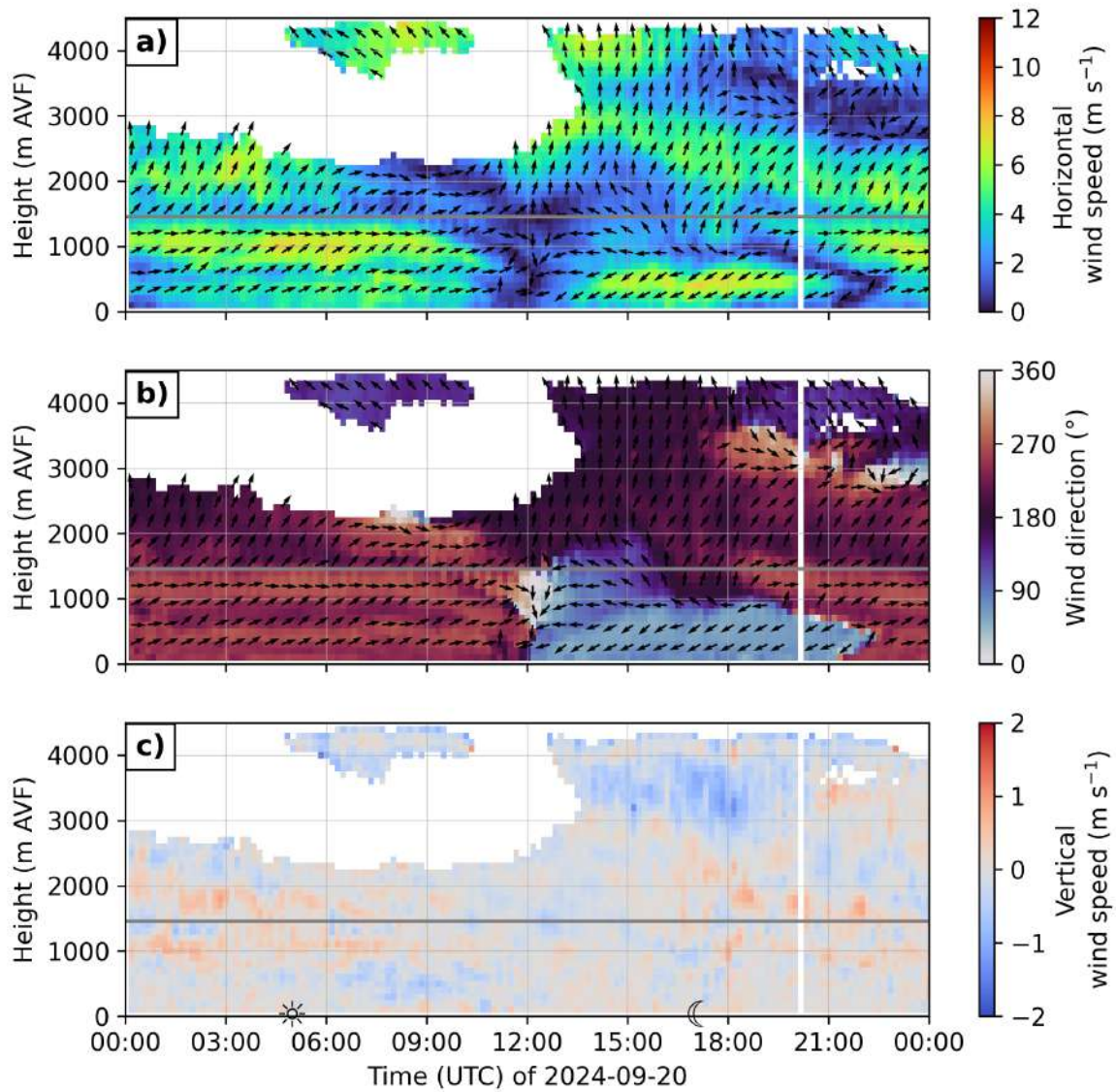
Figure 6.4.: As in Figure 6.2, but for 20 September 2024.
