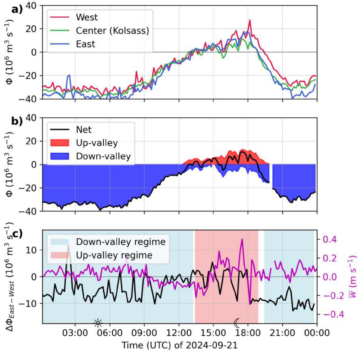
Figure 6.7.: As in Figure 6.3, but for 21 September 2024.
