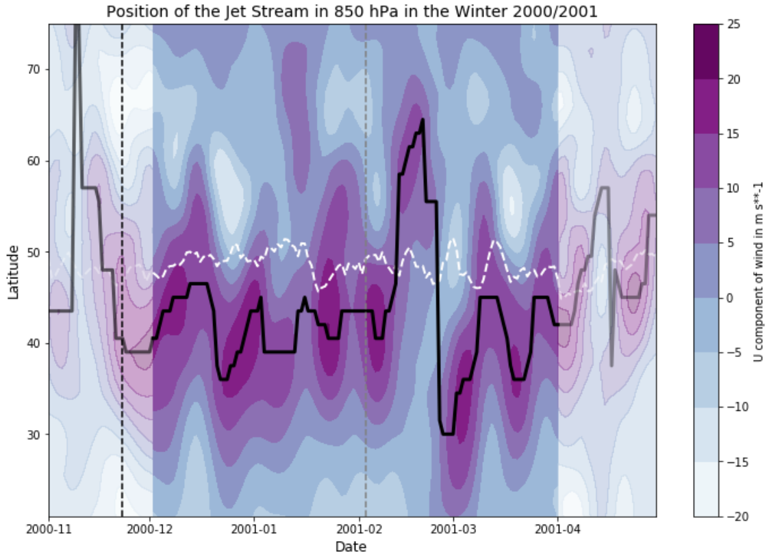
Figure 6.15: Zonal Wind Speed Anomalies during the Winter 2000/2001 based on ERA-Interim. The zonal-wind anomalies in 850 hPa, averaged over 60^{\circ}\text{W} to 0^{\circ}\text{E} are shown as shading in the Hovmöller diagram. The anomalies are filtered using a Lanczos filter with a moving window of 61 days and a cutoff-frequency of 1/10 days. Data on the edges of the timeseries are prone to boundary effects due to the filtering and therefore, shown paler than the unaffected data. The wind maxima are shown as a black solid line. The white dashed line shows the climatological position of the mid-latitudes jet stream. The central date of the first SSW in the winter 2000/2001 is marked with the vertical black dashed line, the central date of the second SSW with the vertical grey dashed line.
