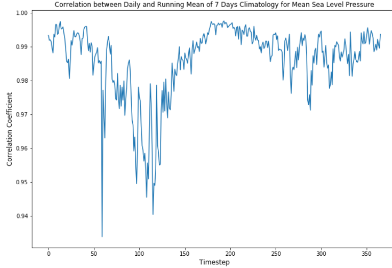
Figure 3.1: Differences between Climatologies Based on ERA-Interim (1979-2019). Correlation of the daily climatology and the 7-day running mean climatology for the mean sea level pressure. The time step on the x-axis of the figure corresponds to the day of year.
