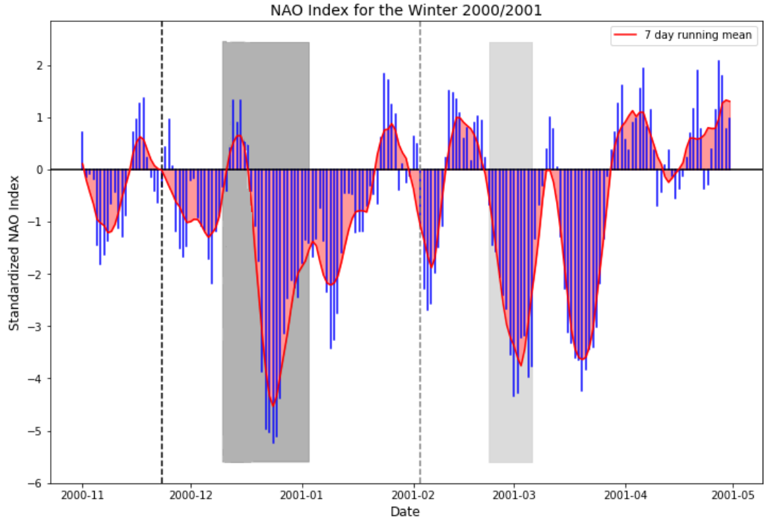
Figure 6.16: NAO Index during the Winter 2000/2001 based on ERA-Interim. Shown is the Zonal Index which is calculated as the standardized mean sea level pressure anomaly difference between a southern box, averaged over 40°W to 0°E and 35°N to 50°N, and a northern box, averaged over 40°W to 0°E and 55°N to 70°N (Leckebusch et al., 2008). The black dashed line marks the central date of the first SSW, the grey dashed line the central date of the second SSW. The period with normalized geopotential height anomalies >1.0 standard deviation associated with the SSWs at surface is shaded in dark grey for the first SSW of the winter 2000/2001 and in light grey for the second SSW of this winter.
