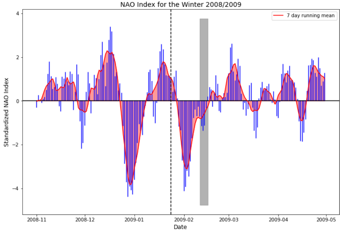
Figure 4.9: NAO Index during the Winter 2008/2009 based on ERA-Interim. Shown is the Zonal Index which is calculated as the standardized mean sea level pressure anomaly difference between a southern box, averaged over 40°W to 0°E and 35°N to 50°N, and a northern box, averaged over 40°W to 0°E and 55°N to 70°N (Leckebusch et al., 2008). The black dashed line marks the central date of the SSW. The period with normalized geopotential height anomalies >1.0 standard deviation associated with the SSW which are present continuously from the stratosphere to the surface, is shaded in dark grey.
