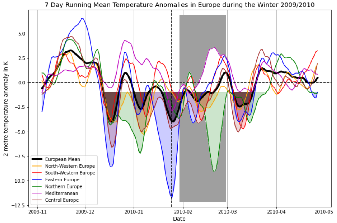
Figure 5.11: 2 Metre Temperature Anomalies during the Winter 2009/2010 based on ERA-Interim.
