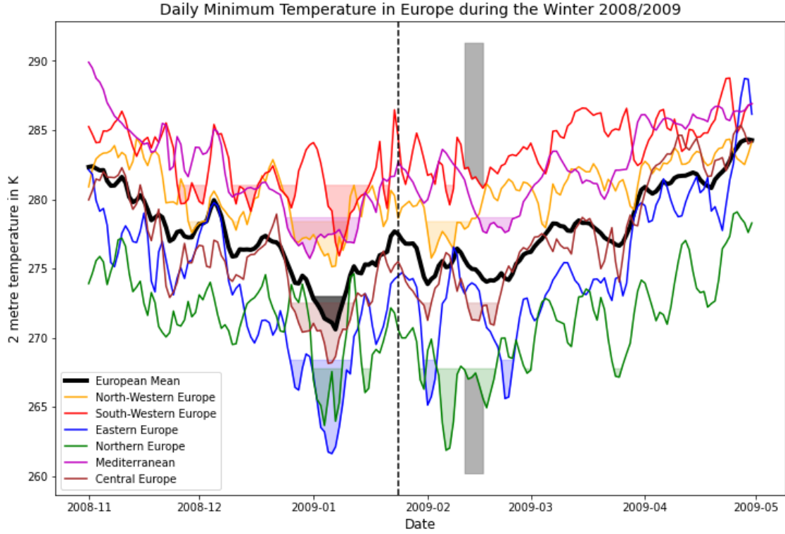
Figure 4.12: 2 Metre Daily Minimum Temperature during the Winter 2008/2009 based on ERA-Interim. Periods of cold waves are defined as at least 3 consecutive days with daily minimum temperatures below the 10 th percentile of the climatological daily minimum temperature (Smid et al., 2019). The climatology is calculated for the period between 1999 and 2019 with a 31 day running mean. The days with cold waves are marked as shading in the respective color. The vertical black dashed line marks the central date of the SSW. The period with normalized geopotential height anomalies >1.0 standard deviation associated with the SSW which are present continuously from the stratosphere to the surface, is shaded in dark grey. The European mean is calculated by averaging between 10°W to 42°E and 35°N to 72°N. The anomalies for north-western Europe between 10°W to 3°E and 45°N to 60°N, for south-western Europe between 10°W to 3°E and 35°N to 45°N, for eastern Europe between 20°E to 42°E and 45°N to 60°N, for northern Europe between 3°E to 42°E and 60°N to 72°N, for central Europe between 3°W to 20°E and 45°N to 60°N and for the Mediterranean between 3°E to 42°E and 35°N to 45°N.
