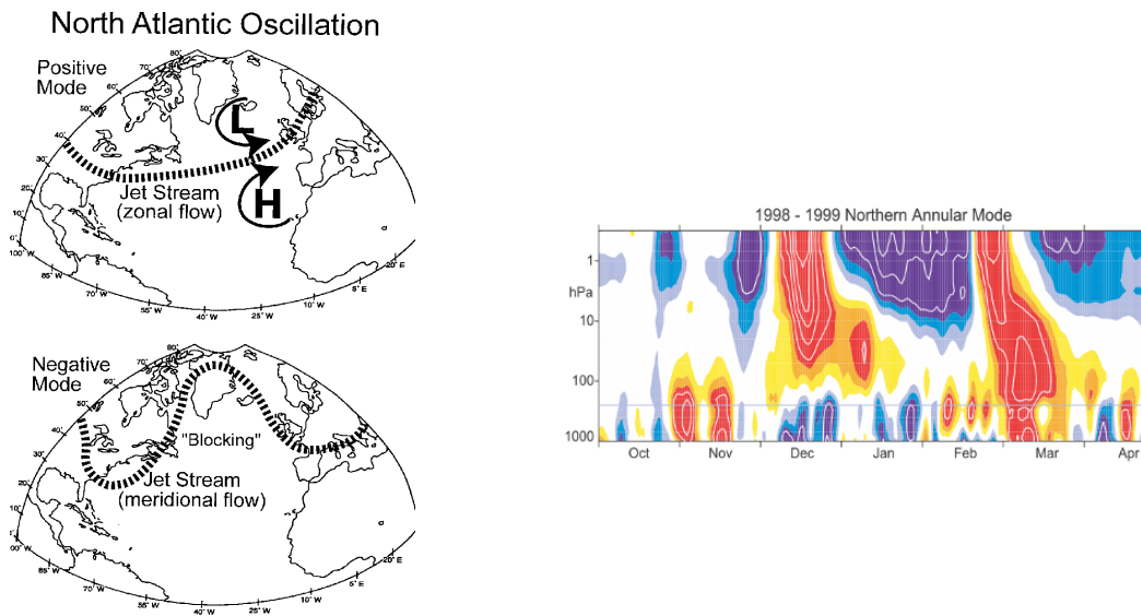
Figure 2.6: Schematic of the NAO Phases and Downward Propagation of Stratospheric AO Signals. Figure 1 of Bradbury et al. (2002) (left): „Schematic Illustration of North Atlantic Atmospheric Conditions During Positive (upper panel) and Negative (lower panel) Phases of the North Atlantic Oscillation (NAO). During positive NAO winters the atmospheric pressure gradient between Iceland and the Azores is at a maximum and the mid-latitude westerlies dominate air circulation throughout the region. During negative NAO winters the Icelandic low is weak and Atlantic blocking occurs more frequently.“ Figure 1 of Baldwin and Dunkerton (2001) (right): „Time-height development of the northern annular mode during the winter of 1998 –1999. The indices have daily resolution and are nondimensional. Blue corresponds to positive values (strong polar vortex), and red corresponds to negative values (weak polar vortex). The contour interval is 0.5, with values between \geq 0.5 and -0.5 unshaded. The thin horizontal line indicates the approximate boundary between the troposphere and the stratosphere.“
