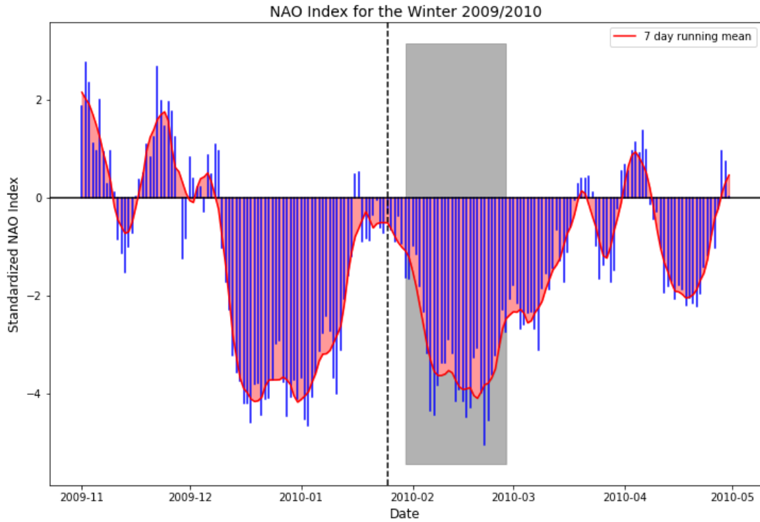
Figure 5.9: NAO Index during the Winter 2009/2010 based on ERA-Interim. Shown is the Zonal Index which is calculated as the standardized mean sea level pressure anomaly difference between a southern box, averaged over 40^{\circ}\text{W} to 0^{\circ}\text{E} and 35^{\circ}\text{N} to 50^{\circ}\text{N} , and a northern box, averaged over 40^{\circ}\text{W} to 0^{\circ}\text{E} and 55^{\circ}\text{N} to 70^{\circ}\text{N} (Leckebusch et al., 2008). The black dashed line marks the central date of the SSW. The period with normalized geopotential height anomalies >1.0 standard deviation associated with the SSW at surface is shaded in dark grey.
