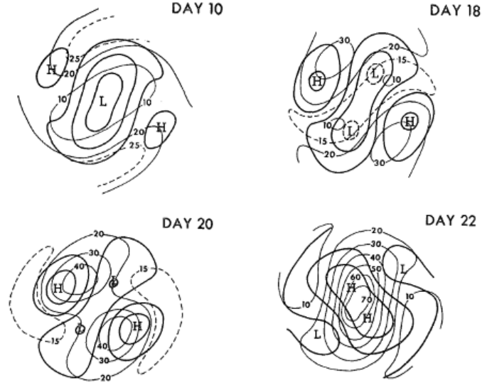
Figure 2.3: Time Evolution of Isobaric Heights and Temperature, Calculated with Matsuno's Model.
