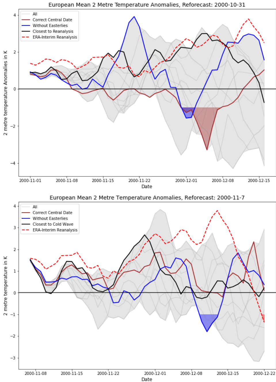
Figure 6.23: 2 Metre Temperature Anomalies of S2S Reforecasts Initialized Before the Central Date of the SSW. In the top plot, the reforecast initialized on 31 October 2000 is shown from 1 November 2000 onwards, in the bottom plot the reforecast initialized on 7 November 2000 is shown. The red dashed line shows the ERA-Interim reanalysis. The European mean is calculated by averaging between 10°W to 42°E and 35°N to 72°N. The data of the first and last 3 days of the reforecasts are prone to boundary effects due to the use of 7-day running mean for the calculation of climatology.
