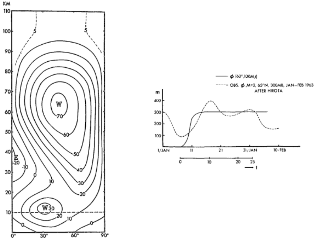
Figure 2.1: Set-Up of Matsuno's Model for a Wavenumber-2 Disturbance in a Typical Northern Hemisphere Wintertime Wind Distribution. Figure 9 of Matsuno (1971) (left): „Initial distribution of zonal winds, adopted as the initial condition for cases C1-C3“. Figure 3 of Matsuno (1971) (right): „The amplitude of waves forced at the lower boundary (solid line). The dashed line shows the observed amplitude of the m=2 wave at 300 mb in January-February 1963 (data from Dr. Hirota).“
