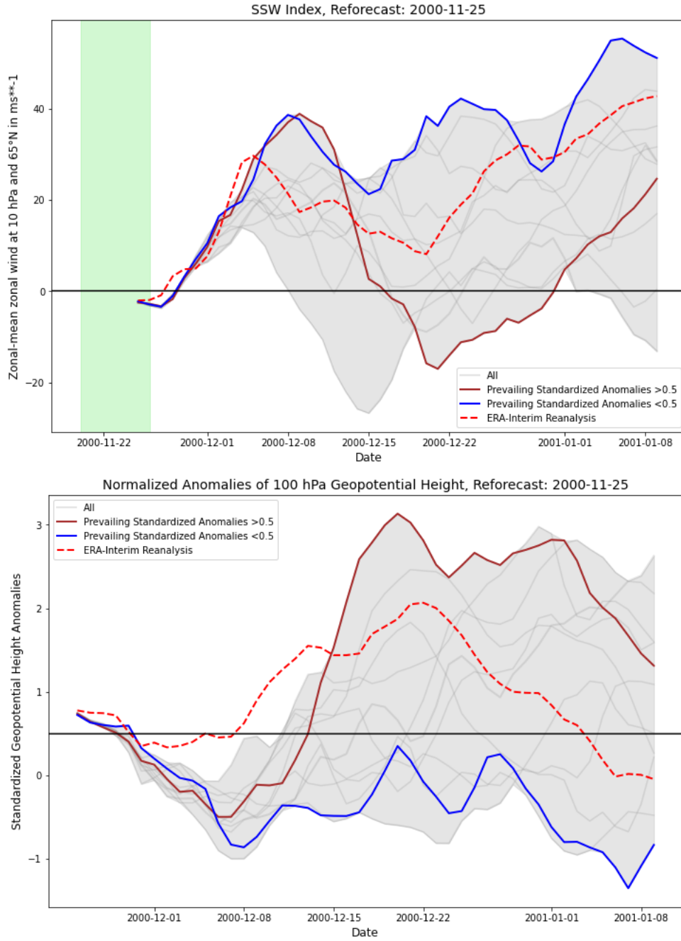
Figure 6.7: SSW Index of the S2S Reforecast Initialized after the Central Date of the SSW and Normalized Geopotential Height Anomalies in 100 hPa. The shaded area shows \pm 3 days around the central date of the SSW event obtained from the ERA-Interim reanalysis. The ERA-Interim reanalysis is shown by the red dashed line (top). The representative members are obtained from the polar-cap averaged 100 hPa normalized geopotential height anomalies (bottom). The data of the first and last 3 days of the 100 hPa standardized geopotential height anomalies reforecast are prone to boundary effects due to the use of 7-day running mean for the calculation of climatology.
