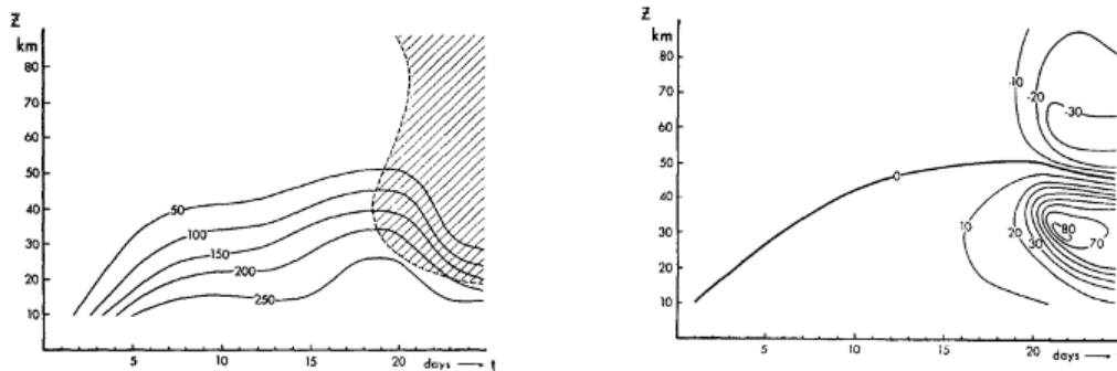
Figure 2.2: Wave Amplitude and Temperature, Calculated with Matsuno's Model. Figure 12 of Matsuno (1971) (left): „Time-height section of the wave amplitude at 60^\circ\text{N} , case C2. Hatched area indicates easterly mean flow.“ Figure 14 of Matsuno (1971) (right): „Time-height section of temperature [deviation ( ^\circ\text{C} ) from the initial temperature] at the pole, case C2.“
