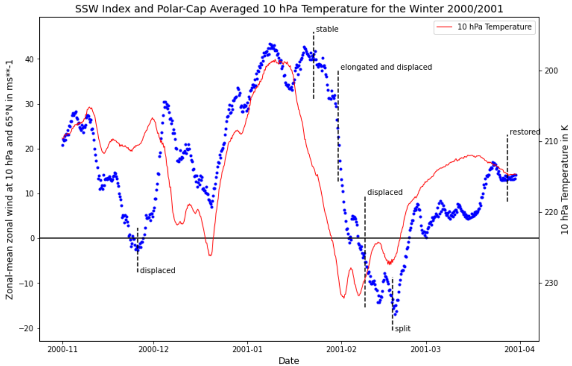
Figure 6.3: SSW Index and Polar-Cap Averaged 10 hPa Temperature for the Winter 2000/2001 based on ERA-Interim. The blue dots show the modified SSW index by Charlton and Polvani (2007) with 65°N instead of 60°N as reference latitude. The red line shows the polar-cap averaged 10 hPa temperature. Days with distinctive shapes of the polar vortex in the 10 hPa geopotential height field are marked.
