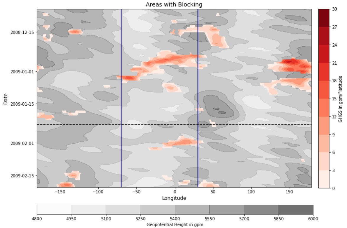
Figure 4.6: Blocking Situation between December 2008 and February 2009 based on ERA-Interim.
