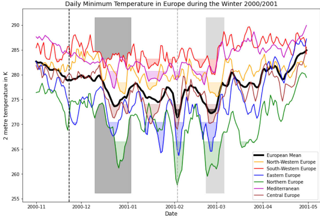
Figure 6.22: 2 Metre Daily Minimum Temperature during the Winter 2000/2001 based on ERA-Interim. Periods of cold waves are defined as at least 3 consecutive days with daily minimum temperatures below the 10 th percentile of the climatological daily minimum temperature (Smid et al., 2019). The climatology is calculated for the period between 1999 and 2019 with a 31 day running mean. The days with cold waves are marked as shading in the respective color. The vertical light grey dashed line marks the central date of the first SSW in the winter 2000/2001, the vertical black line the central date of the second SSW. The period with normalized geopotential height anomalies >1.0 standard deviation associated with the SSW at surface is shaded in dark grey for the first SSW of the winter 2000/2001 and in light grey for the second SSW of this winter. The European mean is calculated by averaging between 10°W to 42°E and 35°N to 72°N. The anomalies for north-western Europe between 10°W to 3°E and 45°N to 60°N, for south-western Europe between 10°W to 3°E and 35°N to 45°N, for eastern Europe between 20°E to 42°E and 45°N to 60°N, for northern Europe between 3°E to 42°E and 60°N to 72°N, for central Europe between 3°W to 20°E and 45°N to 60°N and for the Mediterranean between 3°E to 42°E and 35°N to 45°N.
